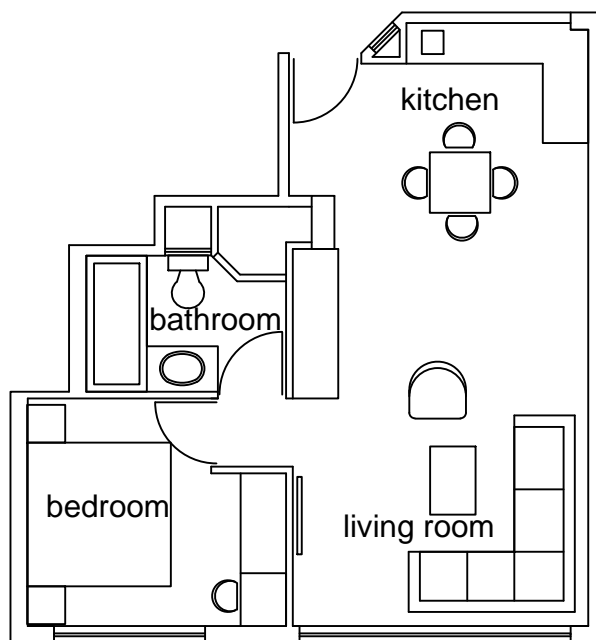
PLAN 1 BEDROOM APARTMENT APARTMENT 1804
