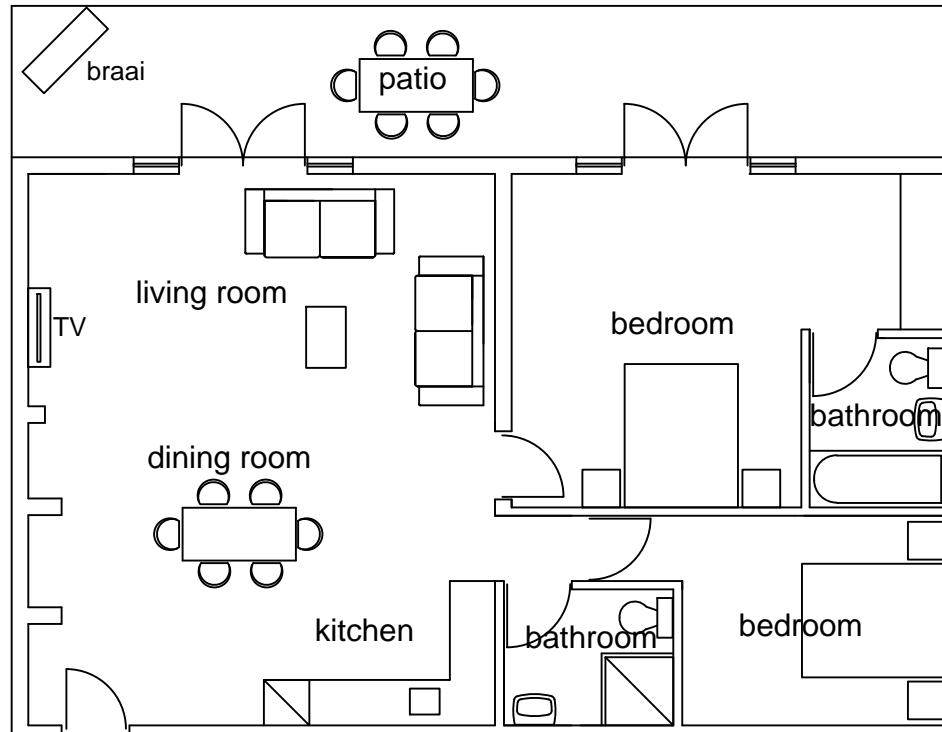
PLAN 2 BEDROOM CHALET - 43
